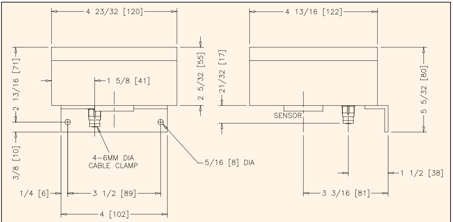
Sensor Dimensions (For reference only)
