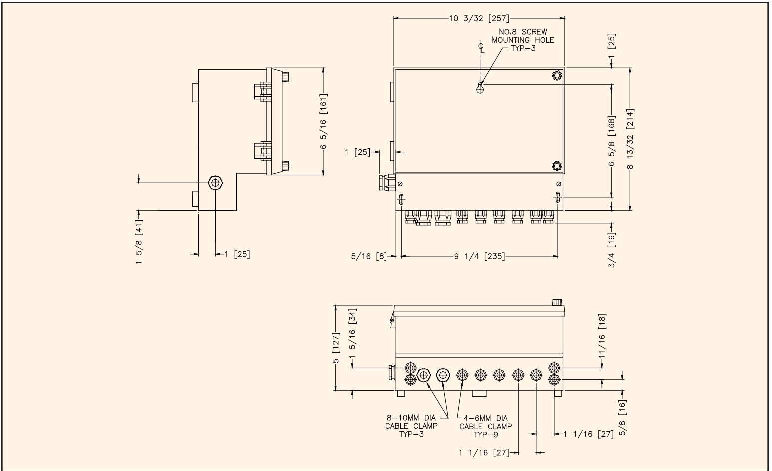
Receiver Dimensions (for reference only)
