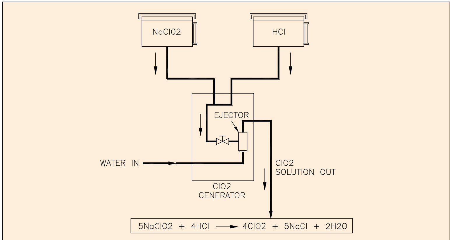
Figure 2 - Flow Diagram
